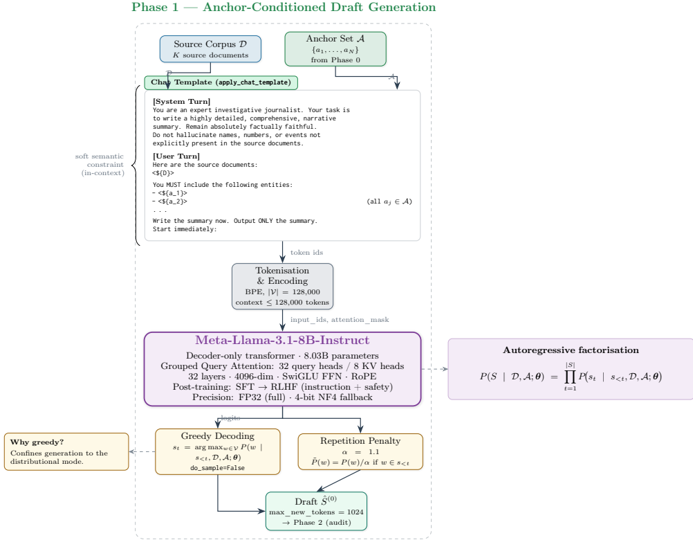
Figure 3: Detailed architectural pipeline for Phase 1: Anchor-Conditioned Draft Generation using Llama-3.1.
